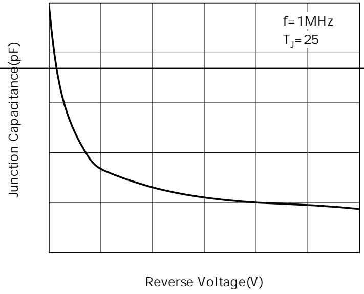
Fig.2: Capacitance Characteristics
